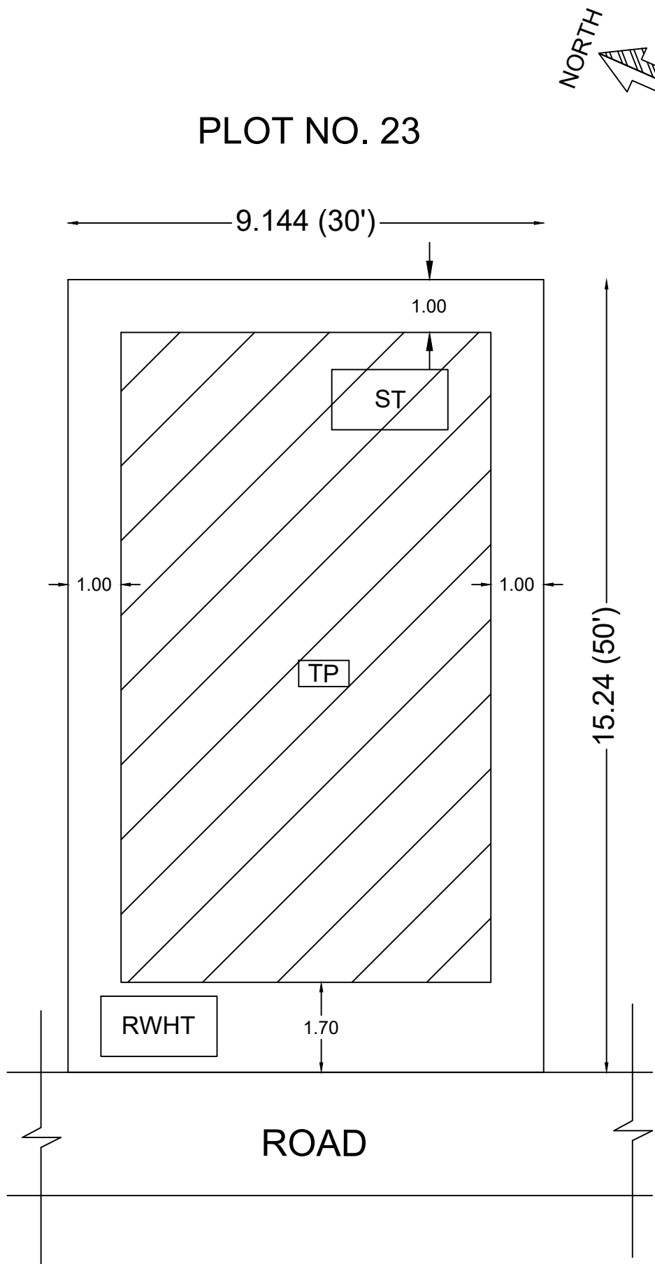
SITE PLAN
