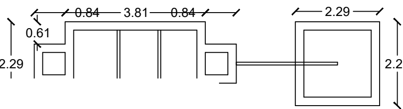
NK AND SOAK PIT (NOT IN SCALE)
