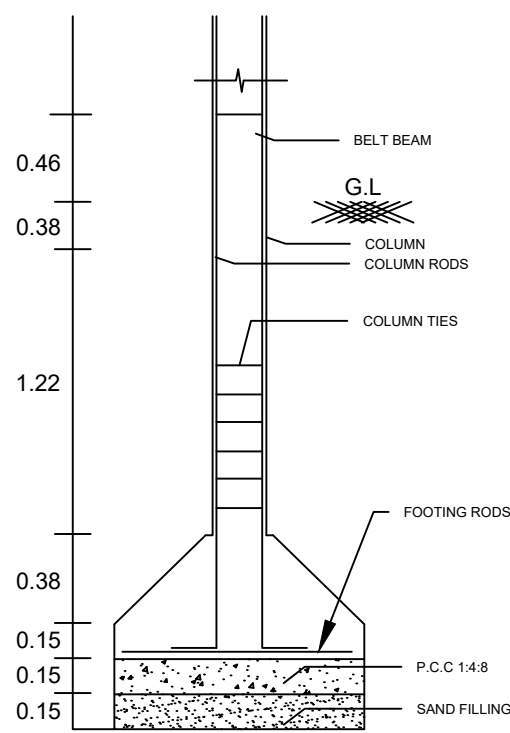
FOUNDATION DETAILS (NOT IN SCALE)
