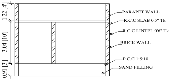
SECTION ON"AB"
