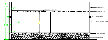
SECTION ON K-S
