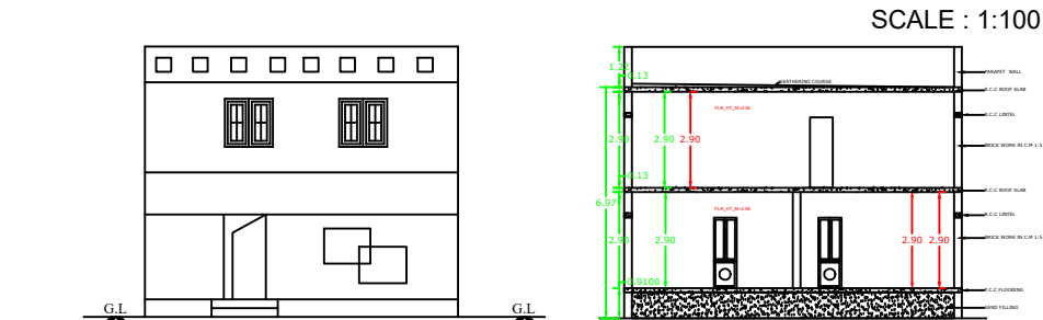
FRONT ELEVATION
