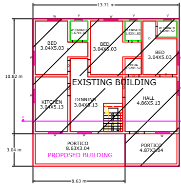
EXISTING GROUND FLOOR PLAN (Already approved)
