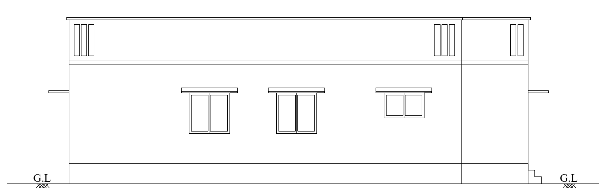
FRONT ELEVATION
