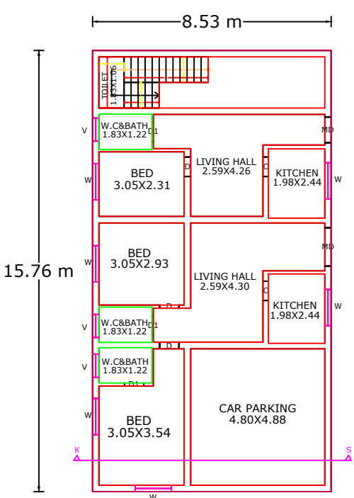
PORPOSED GROUND FLOOR PLAN
