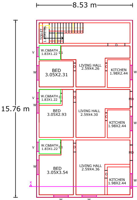
PORPOSED FIRST FLOOR PLAN
