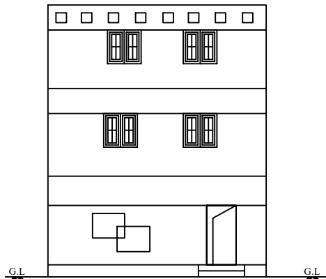
FRONT ELEVATION
