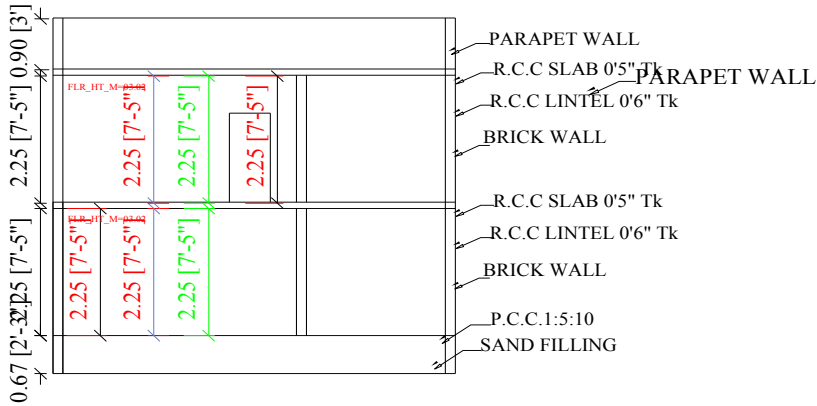
SECTION ON"AB"
