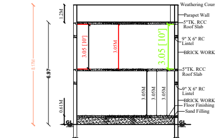
SECTION ON "SR"
