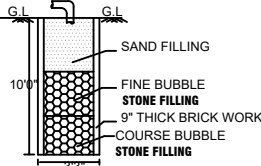
RAIN WATER COLLECTION TANK
