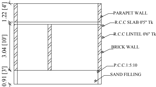
SECTION ON"AB"
