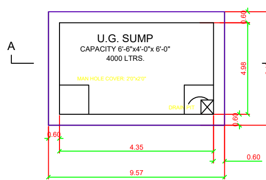
SUMP DETAIL
