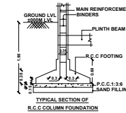
TYPICAL SECTION OF R.C.C. COLUMN FOUNDATION
