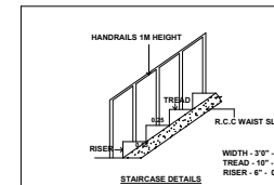
STAIRCASE DETAILS
