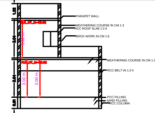
SECTIONON-"AA"&"BB"
