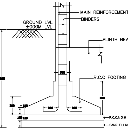
TYPICAL SECTION OF R.C.C COLUMN FOUNDATION SCALE : 1" = 2'-0"
