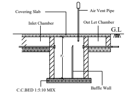
SECTION ON S.Tank
