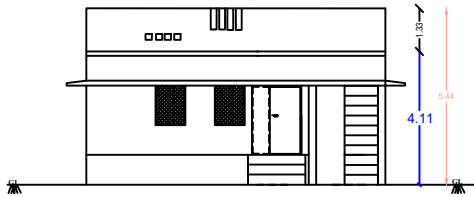
ELEVATION FACING EAST
