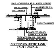
SECTION ON SEPTIC TANK (NOT TO SCALE)
