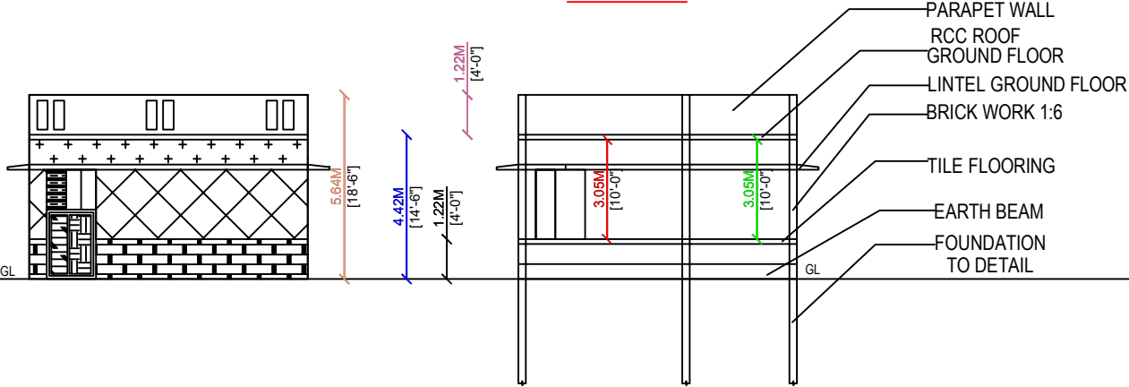
FRONT ELEVATION.
