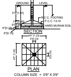
PERCOLATION PIT
