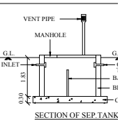
SECTION OF SEP. TANK
