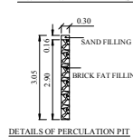
DETAILS OF PERCOLATION PIT
