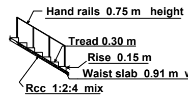
Staircase Details
