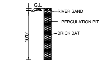
PERCUSSION PIT
