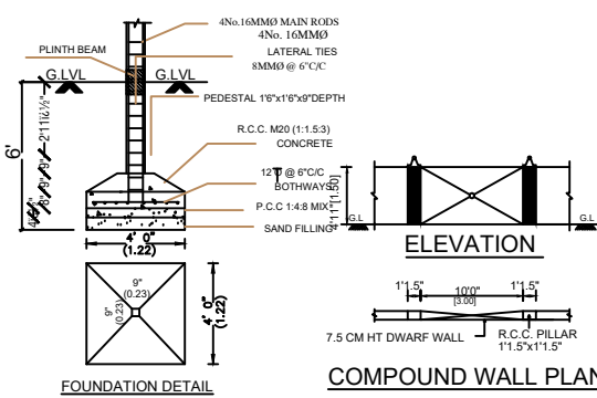
FOUNDATION DETAIL
