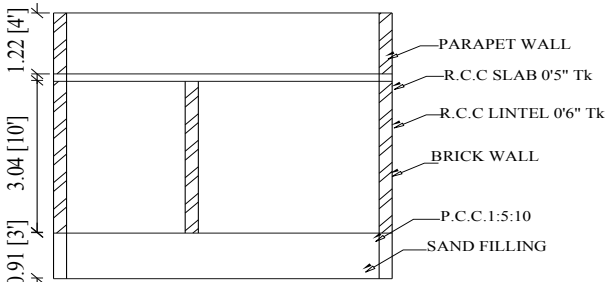
SECTION ON"AB"
