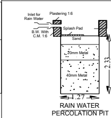
RAIN WATER PERCOLATION PIT
