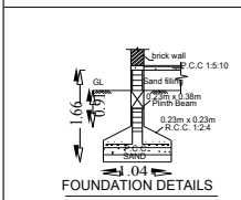
FOUNDATION DETAILS
