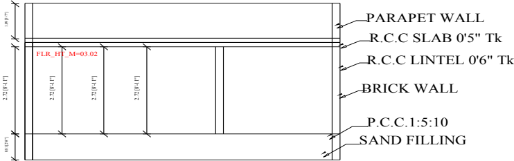
SECTION ON"AB"
