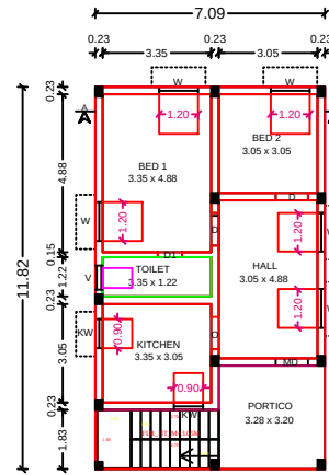
GROUND FLOOR PLAN (EAST FACING)
