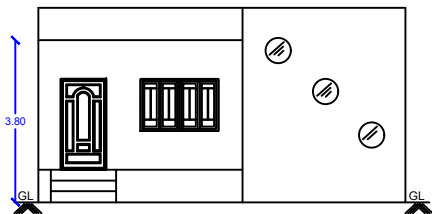
FRONT ELEVATION (NORTH FACING)
