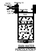
RAIN WATER PERCOLATION PIT
