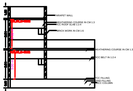
SECTION ON-"AA" & "BB"
