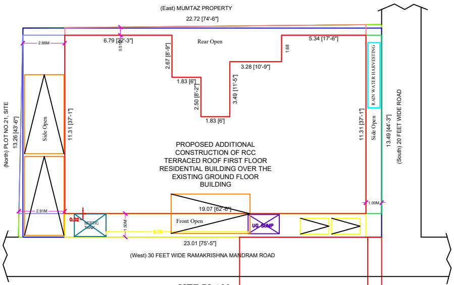
SITE PLAN
