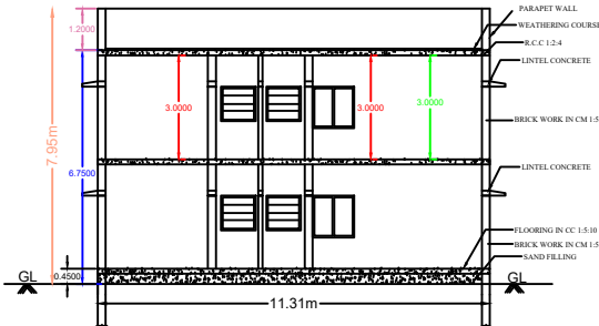
SECTION AB
