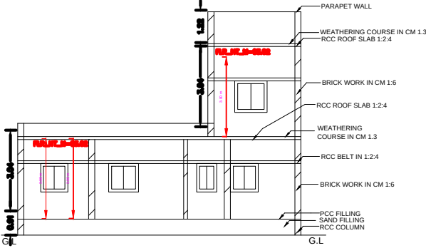
SECTION ON-AA&BB
