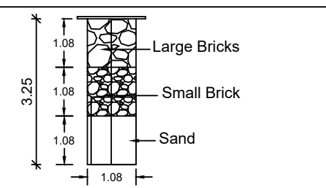
SECTION OF RAIN WATER COLLECTION PITS (NTS)
