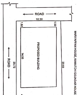
SITE PLAN
