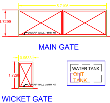
WICKET GATE
