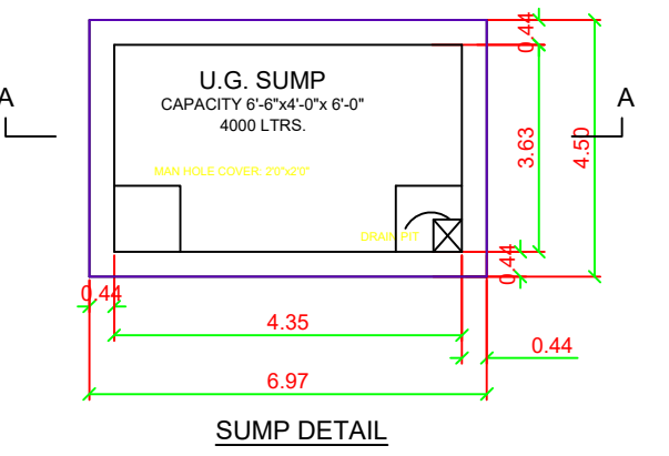
SUMP DETAIL
