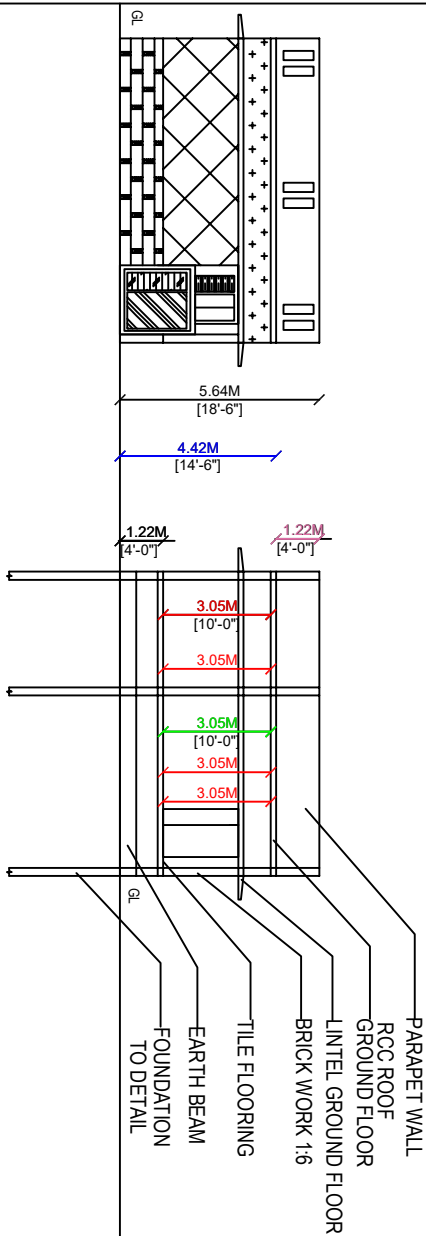
FRONT ELEVATION.
