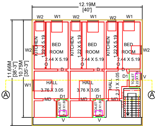
PROPOSED FIRST FLOOR PLAN NORTH FACING
