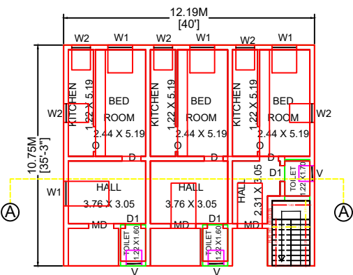
PROPOSED GROUND FLOOR PLAN NORTH FACING
