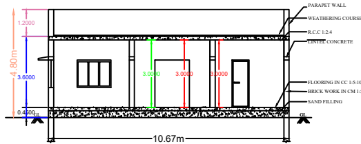
SECTION AB
