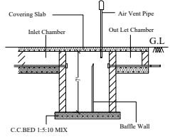
SECTION ON S.Tank
