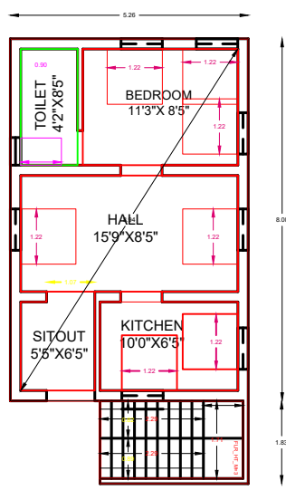
GROUND FLOOR PLAN(EXT) [SOUTH FACING]
