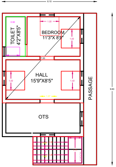
FIRST FLOOR PLAN(PRO)
