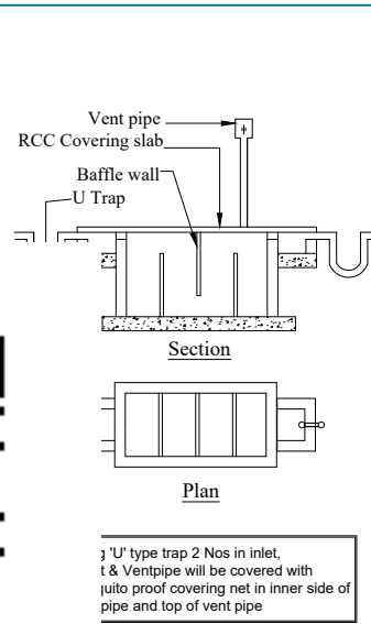
Water Tank With U Trap Not To Scale
