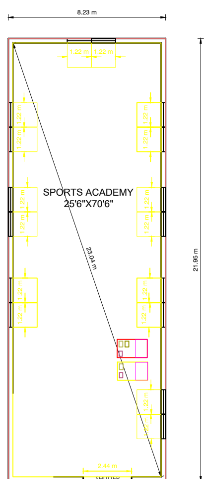
GROUND FLOOR PLAN [EAST FACING]
