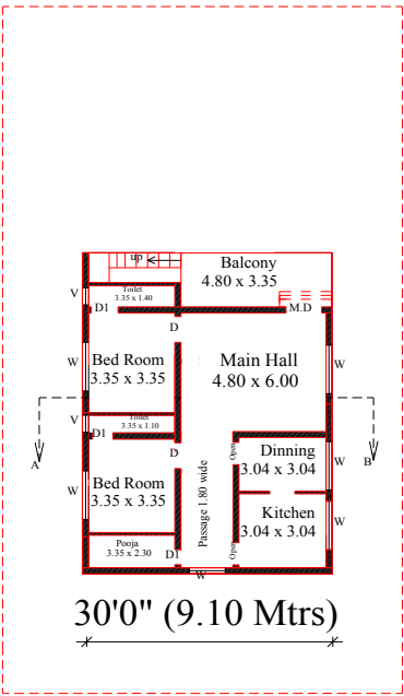
Pro.First Floor
