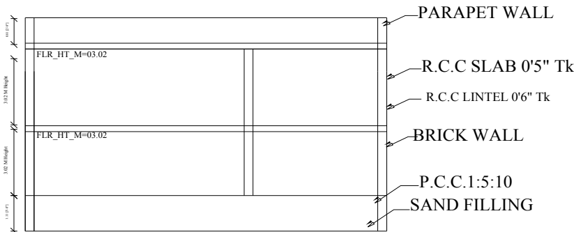
SECTION ON"AB"
