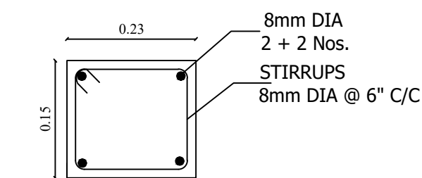
LINTEL BEAM SECTION
