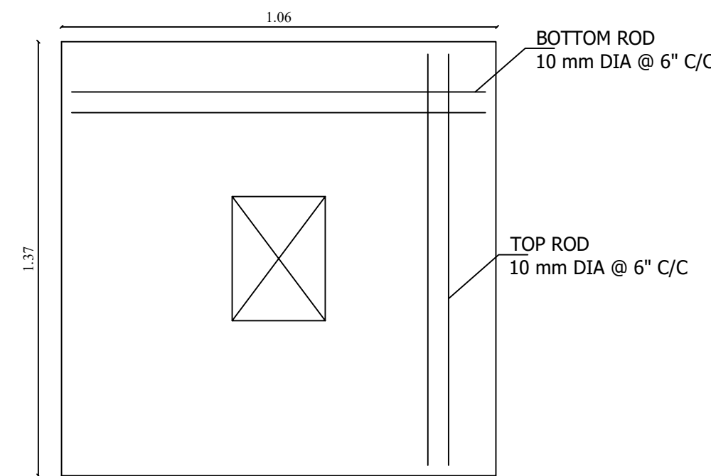
FOOTING PLAN
