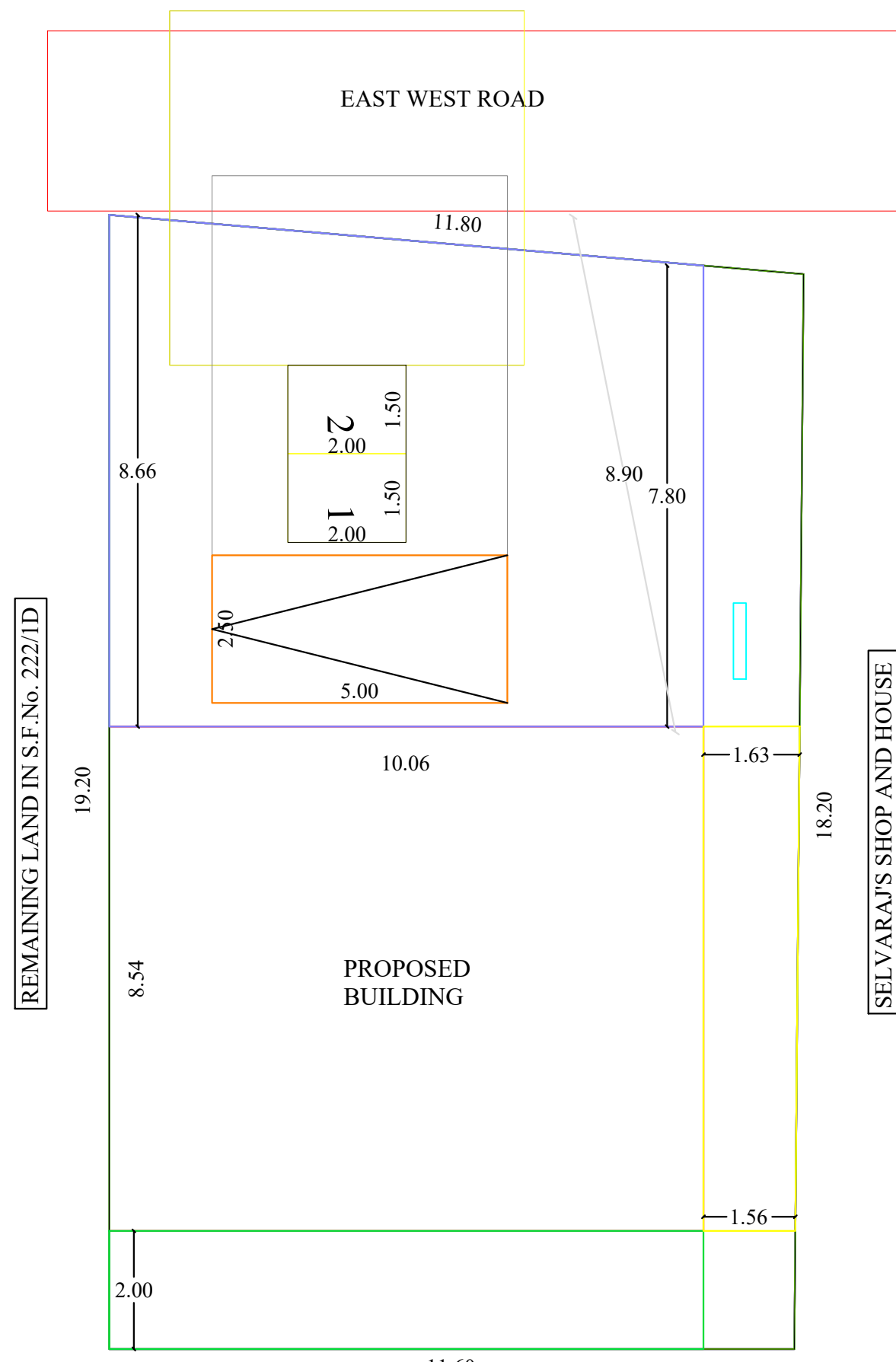
SITE PLAN
