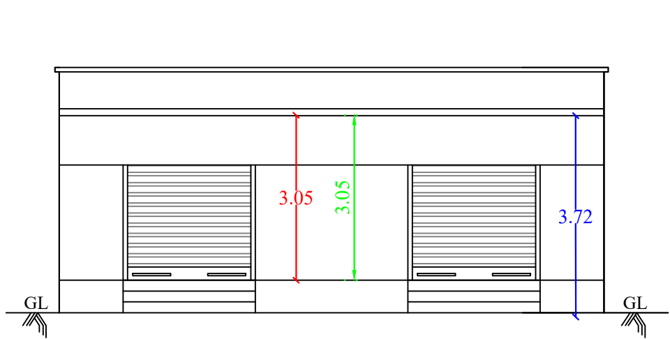
FRONT ELEVATION
