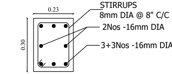
COLUMN PLAN
