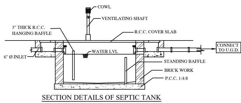
SECTION DETAILS OF SEPTIC TANK
