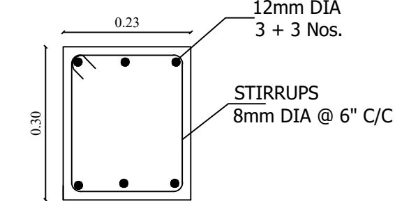
ROOF BEAM SECTION
