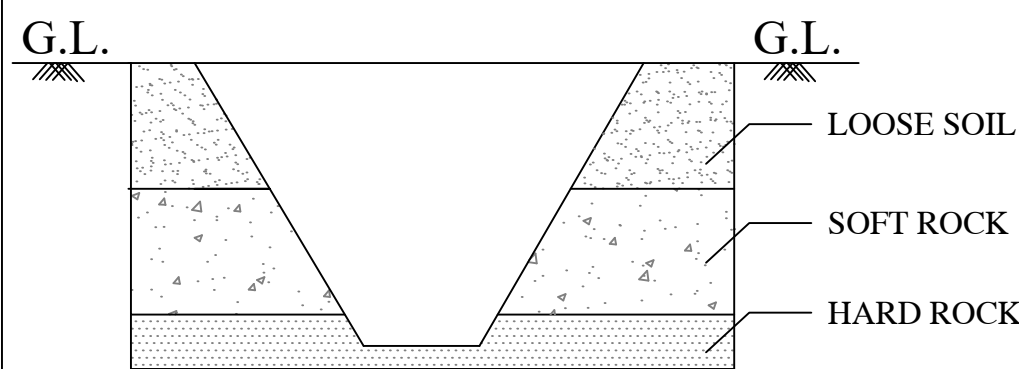
TRIAL PIT
