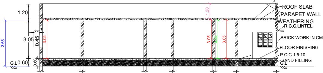
SECTION ON SS
