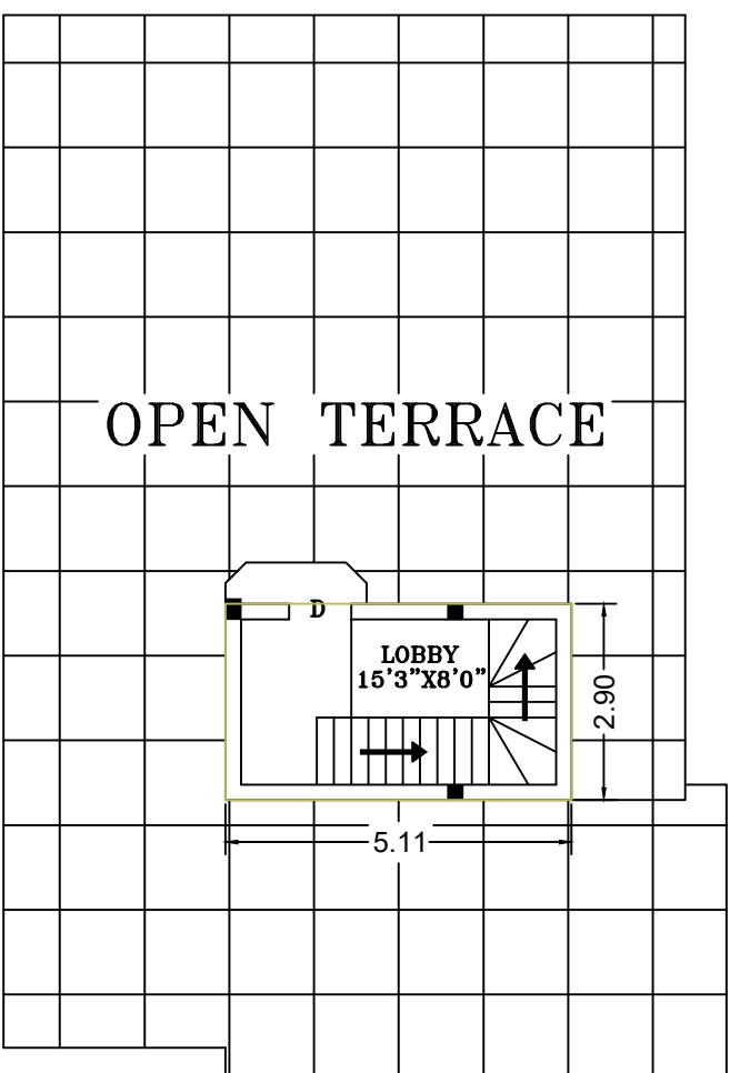
HEAD ROOM PLAN
