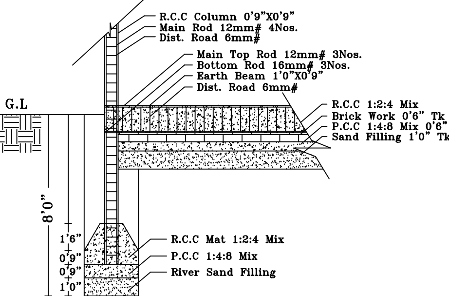
FOUNDATION DETAILS
