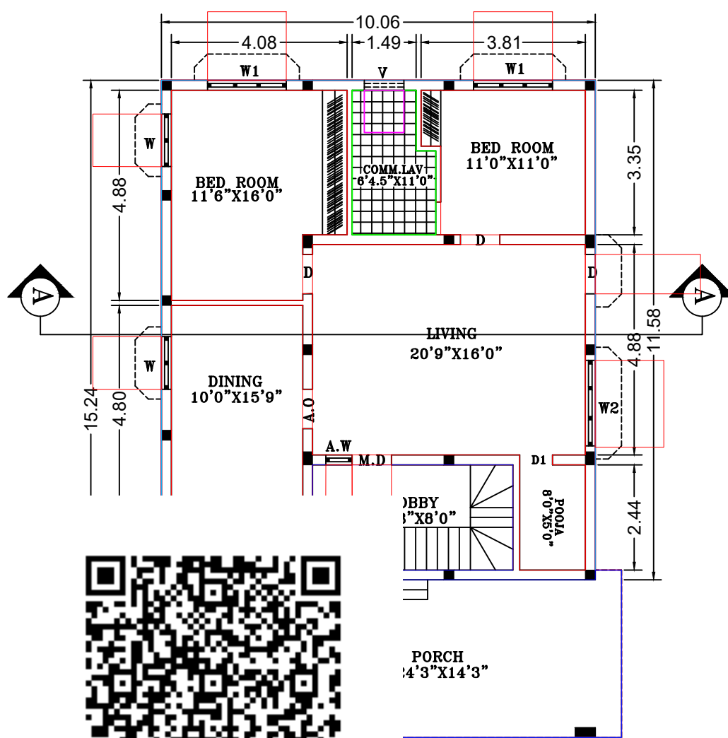
FLOOR PLAN
