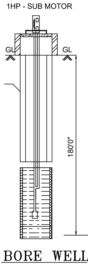
BORE WELL
