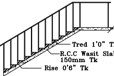
STEPS DETAILS
