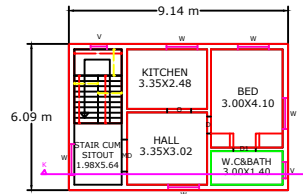
EXISTING FIRST FLOOR PLAN (Already approved)
