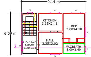
PROPOSED SECOND FLOOR PLAN
