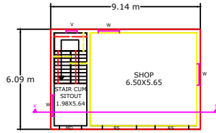
EXISTING GROUND FLOOR PLAN (Already approved)
