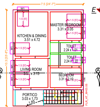
GROUND FLOOR PLAN (1 DWELLING UNIT)
