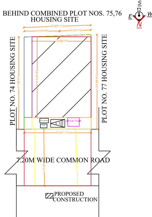
SITE PLAN FOR PLOT NO. 75, 76 @ SEMMOZHI NAGAR
