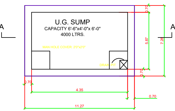
SUMP DETAIL
