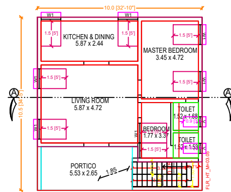
GROUND FLOOR PLAN (1 DWELLING UNIT)
