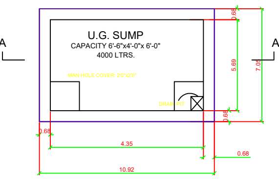
SUMP DETAIL
