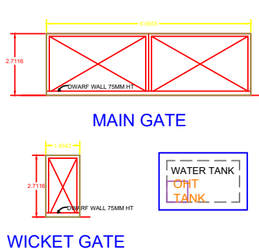
WICKET GATE
