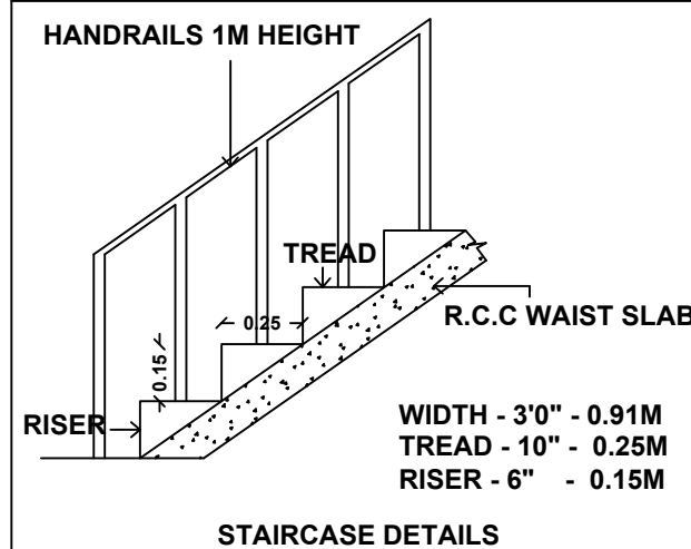
STAIRCASE DETAILS
