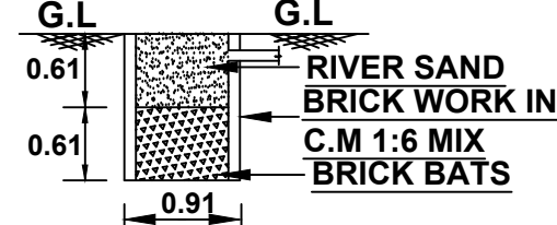
. SECTION ON RAIN WATER COLLECTION TUB .
