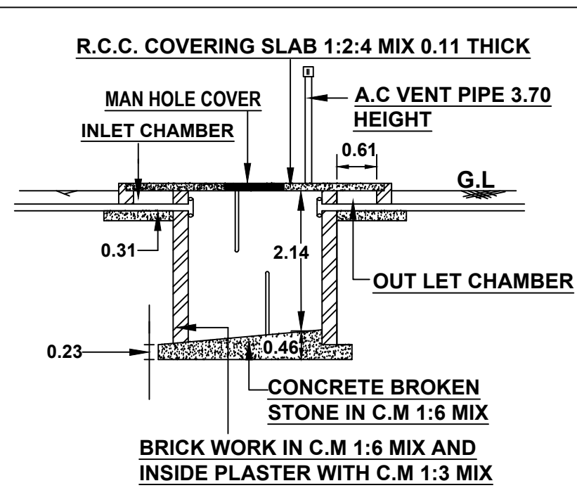
.SECTION ON SEPTIC TANK .
