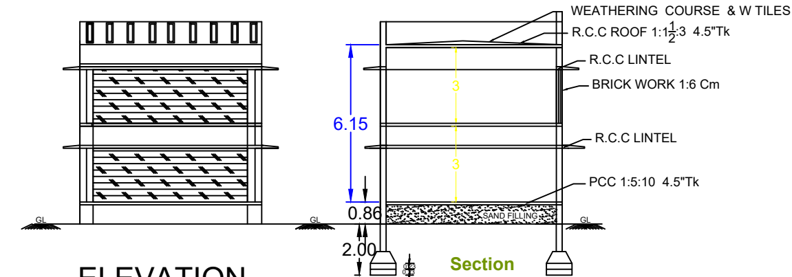
CUT SECTION ON AB
