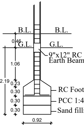
FOUNDATION DETAILS
