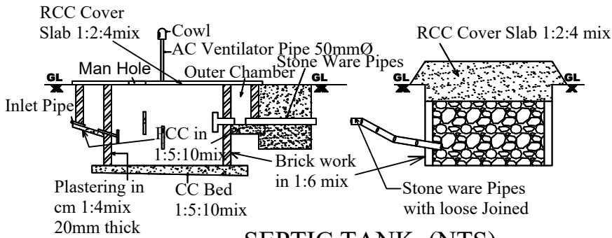
SEPTIC TANK (NTS)
