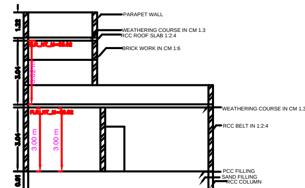
SECTION ON-"AA" & "BB"
